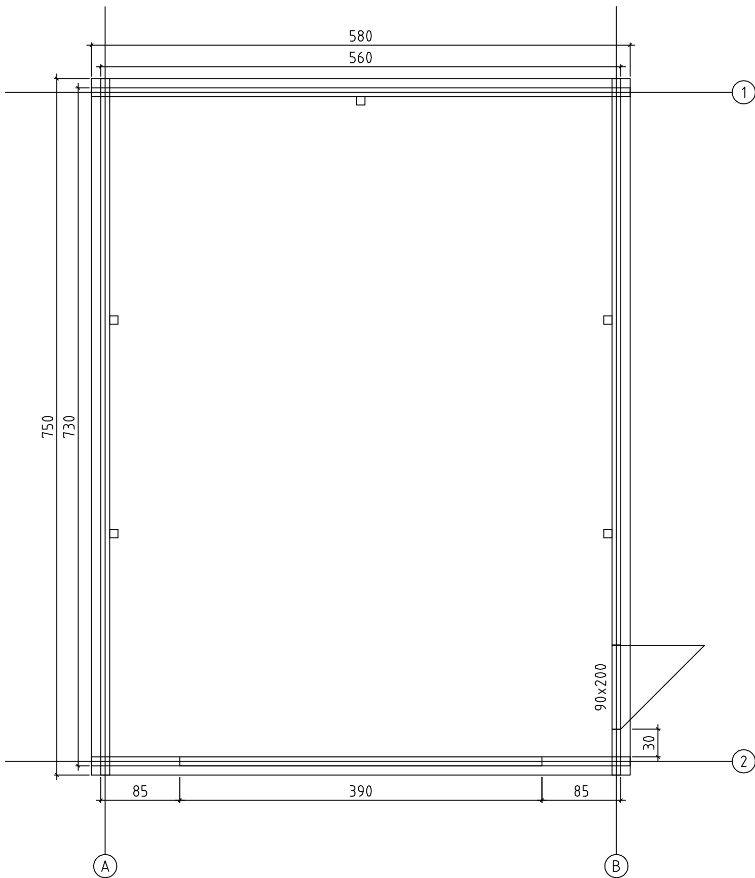
floor plan
